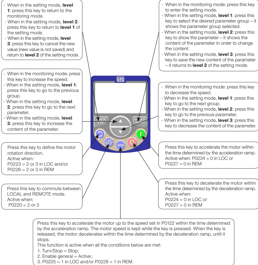
Figure 4.1: HMI Keys
