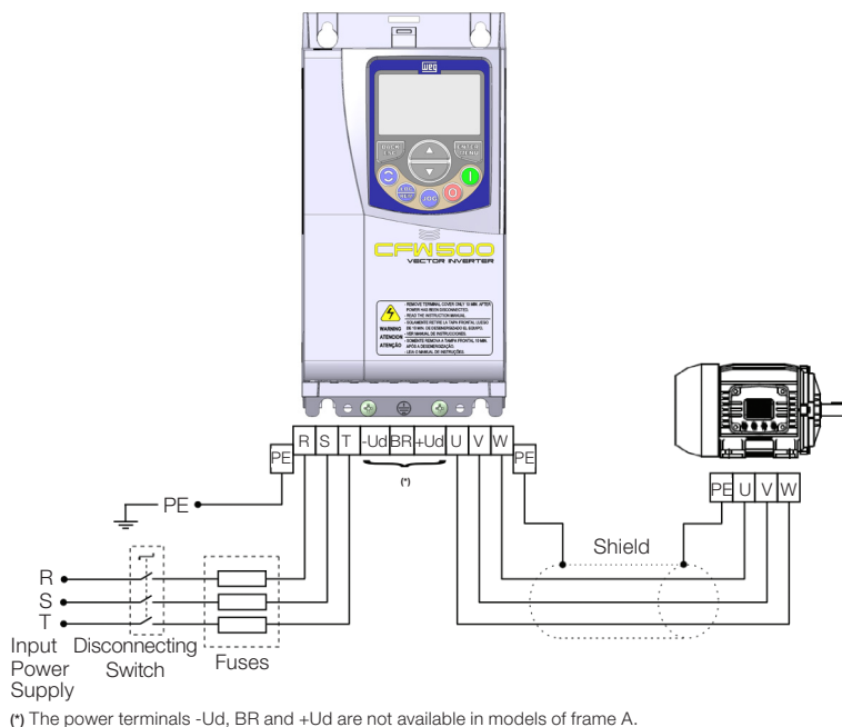
Figure 3.1: Power and grounding connections
