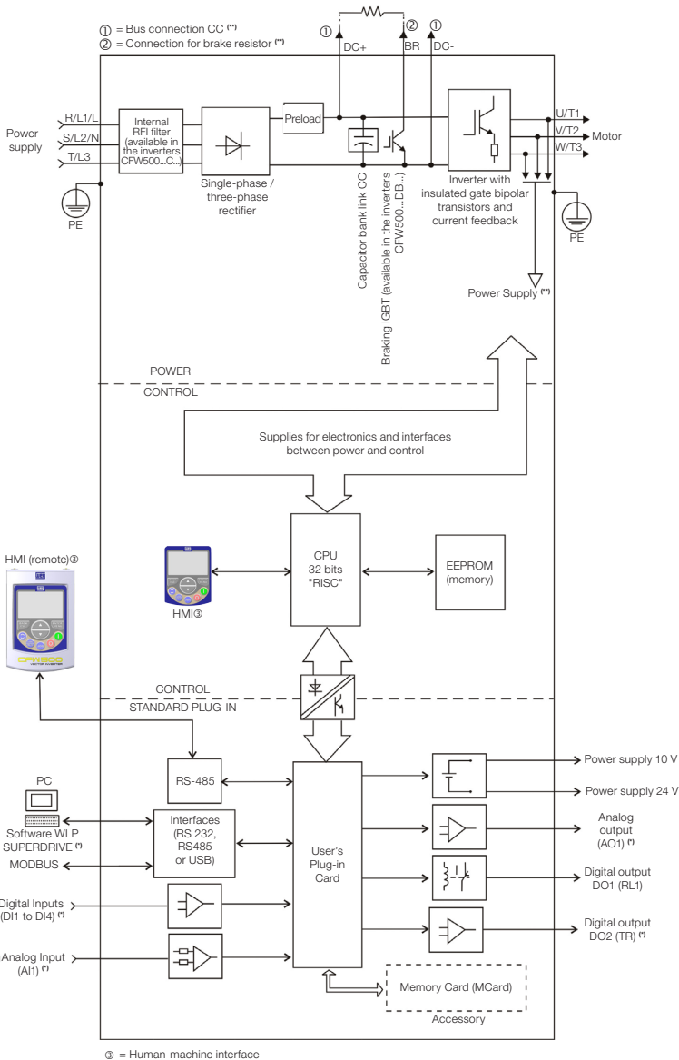
Figure 2.1: Block diagram of CFW500
