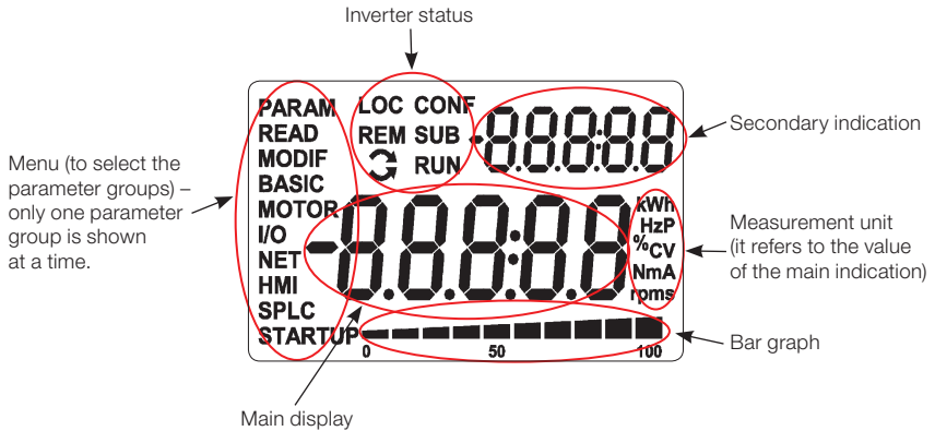
Figure 4.2: Display fields
